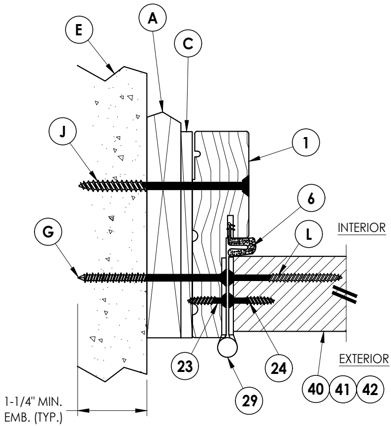
2 5 HORIZONTAL CROSS SECTION Shown w/ 1X sub-buck
