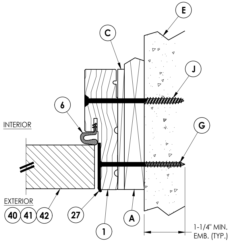
3 5 HORIZONTAL CROSS SECTION Shown w/ 1X sub-buck
