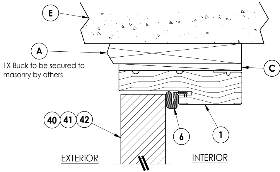
1 5 VERTICAL CROSS SECTION Shown w/ 1X sub-buck
